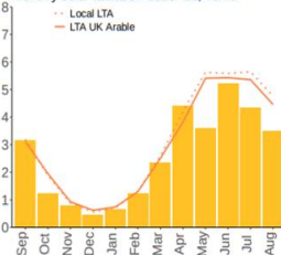
Monthly solar radiation 2020-21, TJ/ha
